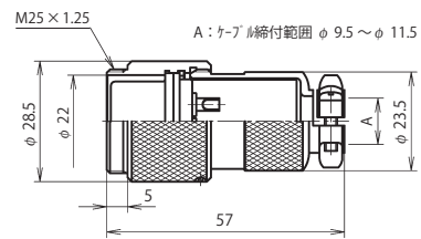
NCS-25 ■ -AdF
