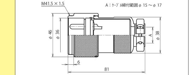
NCS-40 ■ -Ad
