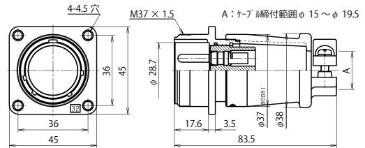
NJC-32 ■ -Ad(F)M
